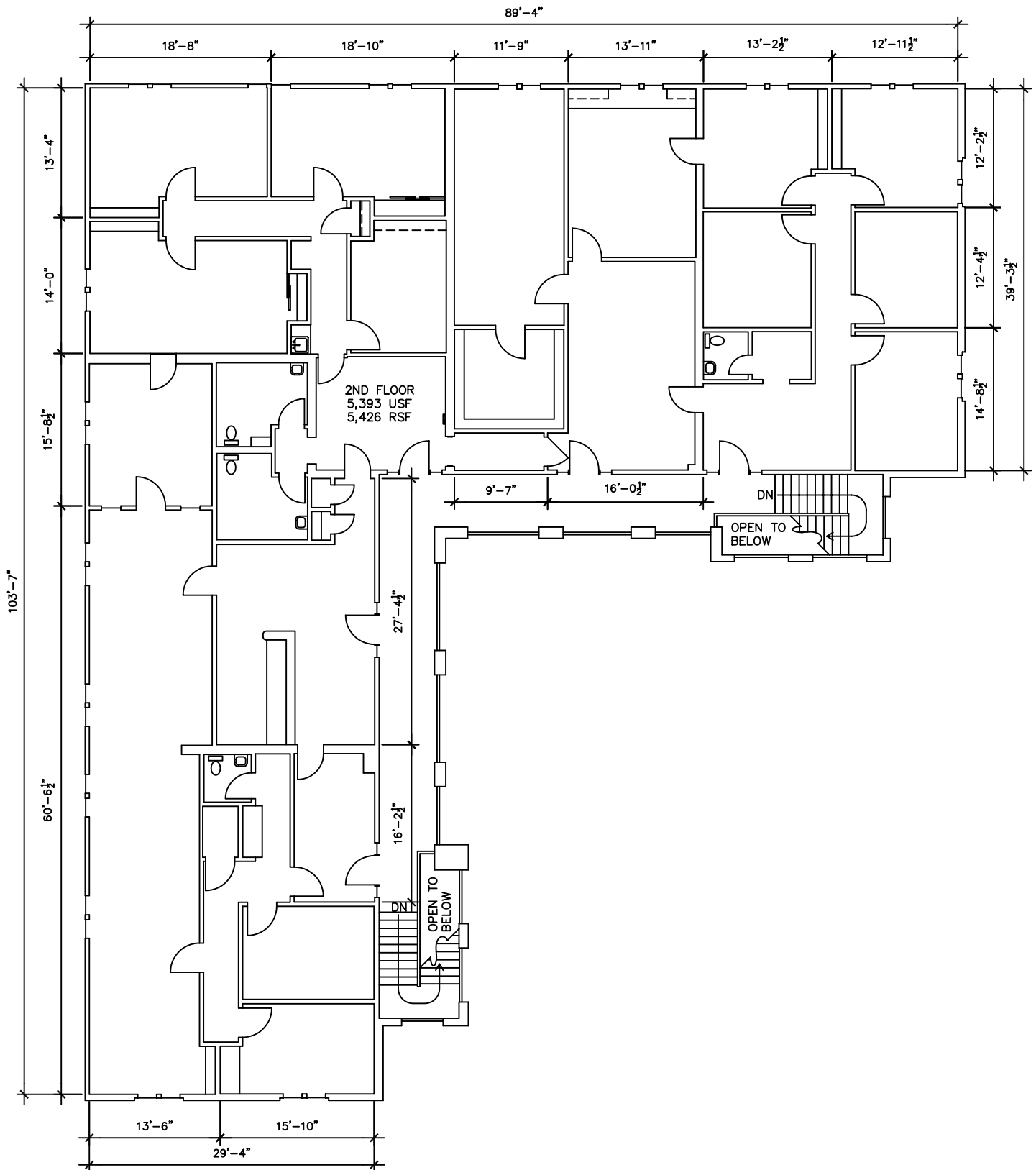
○ SECOND FLOOR
