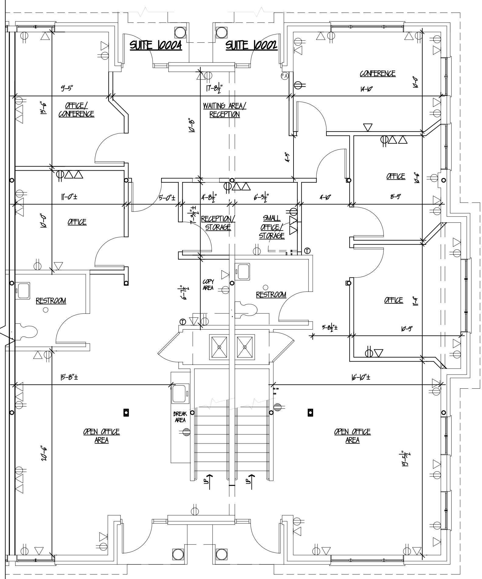
1 A1 1ST FLOOR PLAN - UNITS 10002 - 10004 ↑
